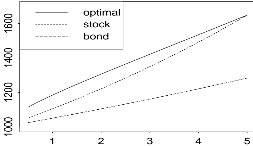
Figure 2: Expected terminal wealth of different investment strategies depending on the time horizon T , 0 < T \leq 5 . The parameters are d = 1 , r = 0.05 , b = 0.1 , \sigma = 0.2 , and \alpha = 0.05 . As the upper bound C of the CaR we used \text{CaR}(1000, 1, 5) , the CaR of the pure stock strategy with time horizon T = 5 .
