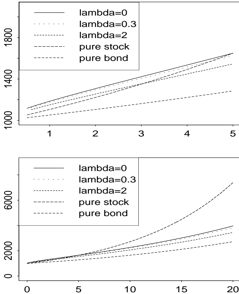
Figure 8: Wealth corresponding to the optimal portfolios for Brownian motion with and without jumps depending on the time horizon T , 0 < T \leq 5 (top) and 0 < T \leq 20 (bottom). The parameters are the same as in Figure 7. The possible jump size is again \beta = -0.1 .
