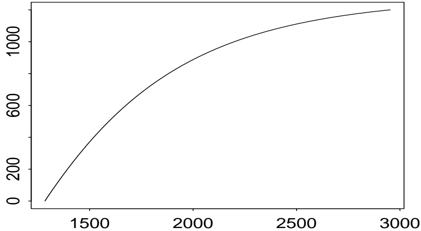
Figure 5: Mean-CaR efficient frontier with the mean on the horizontal axis and the CaR on the vertical axis. The parameters are the same as in Figure 2.
