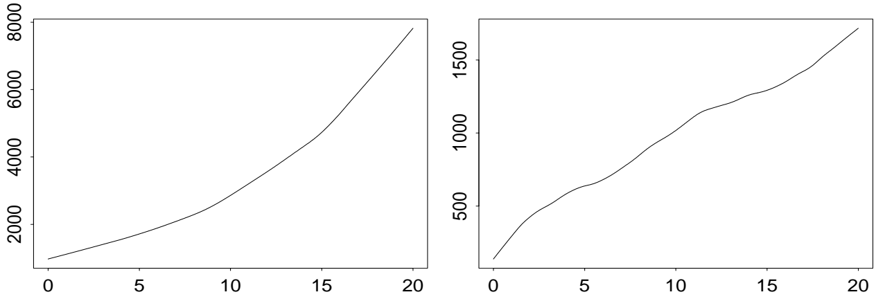
Figure 10: Left: Estimated mean wealth EX^\pi(T) for \pi = 1 , 0 < T \leq 20 , based on N = 100 simulations. Right: Corresponding CaR. We used the same parameters as in Figure 9.
