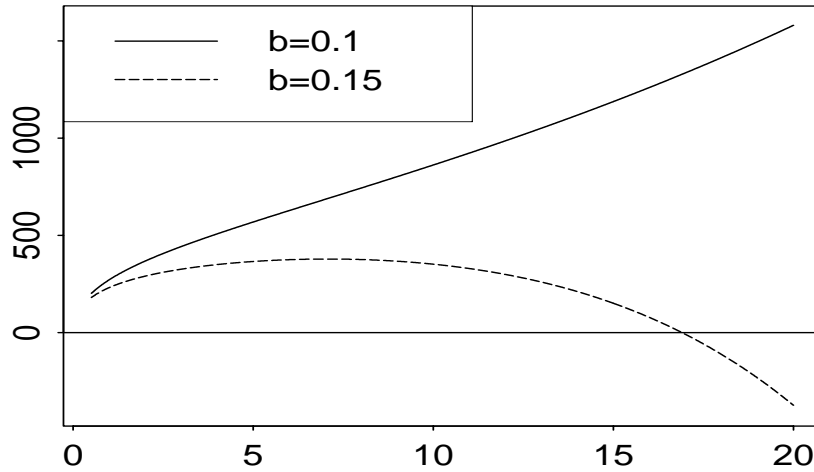
Figure 1: \text{CaR}(1000, 1, T) of the pure stock portfolio (one risky asset only) for different appreciation rates as a function of the planning horizon T ; 0 < T \leq 20 . The volatility is \sigma = 0.2 . The riskless rate is r = 0.05 .
