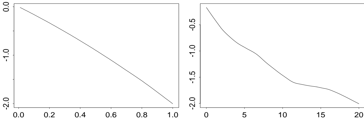
Figure 12: Left: Estimated \widehat{z}_\alpha(\pi) as function of the portfolio \pi , 0 < \pi \leq 1 , for T = 20 , based on N = 100 simulations. Right: The same estimate as on the left-hand side, now as function of the time horizon T , 0 < T \leq 20 , for \pi = 1 , based on N = 100 simulations. The parameters are the same as in Figure 9.
