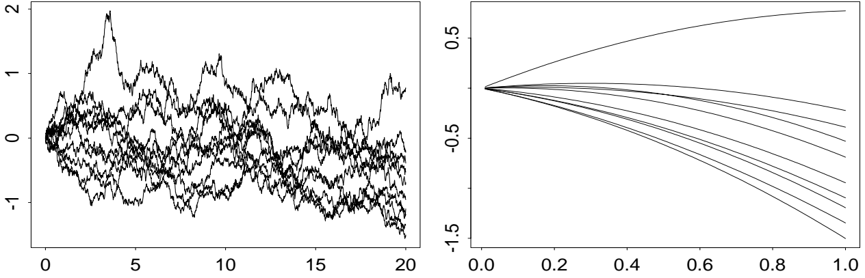
Figure 9: Ten sample paths of (\tilde{Y}(t))_{0 \leq t \leq 20} for \pi = 1 (left) and ten sample paths of \tilde{Y}^\pi(20) for \pi \in (0, 1) (right) for parameter values x = 1000, r = 0.05, b = 0.10, \psi = 4, \lambda = 0, \sigma = 0.05 and u = 5 .
