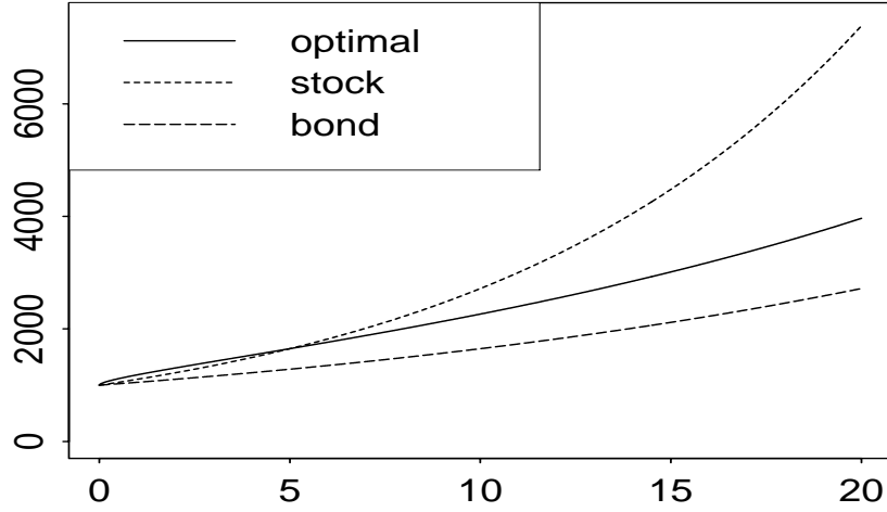
Figure 3: Expected terminal wealth of different investment strategies depending on the time horizon T , 0 \leq T \leq 20 . The parameters are d = 1 , r = 0.05 , b = 0.1 , \sigma = 0.2 , and \alpha = 0.05 . As the upper bound C of the CaR we used \text{CaR}(1000, 1, 5) , the CaR of the pure stock strategy with time horizon T = 5 .
