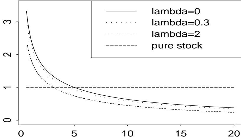
Figure 7: Optimal portfolios for Brownian motion with and without jumps depending on the time horizon T , 0 < T \leq 20 . The basic parameters are the same as in Figure 2. The possible jump size is \beta = -0.1 .
