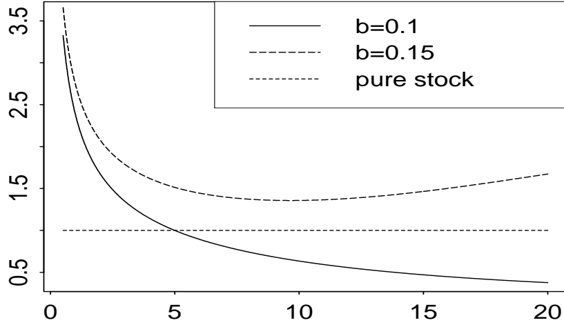
Figure 4: For the same parameters as in Figure 2 and different appreciation rates the figure shows the optimal portfolio and the pure stock portfolio.
