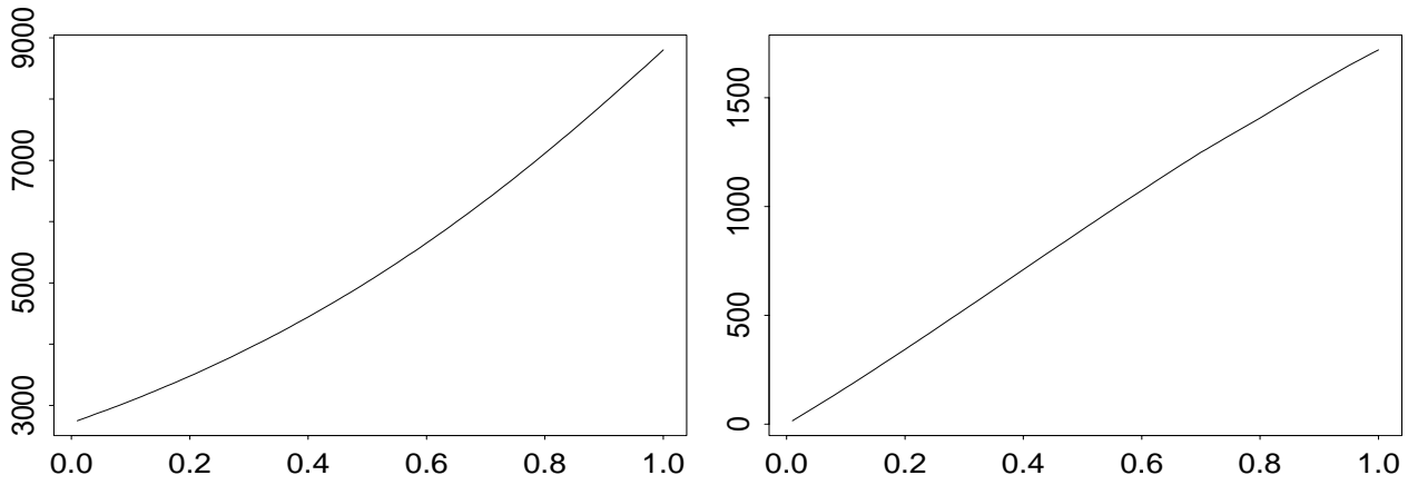
Figure 11: Estimated expected terminal wealth (left) and the corresponding CaR (right) as functions of the portfolio \pi for the GCIR model for T=20 and the same parameters as in Figure 9 (based on N=100 simulations). The expected terminal wealth and the CaR for the GCIR model increase for all \pi \in (0, 1) .
