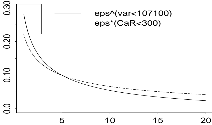
Figure 6: \hat{\varepsilon} and \varepsilon^* as functions of the time horizon; 0 < T \leq 20 . The parameters are the same as in Figure 2.
