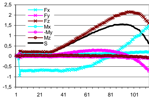
Figure 4: Forces F_x , F_y , F_z , moments M_x , M_y , M_z , and observation curve S of a direct E/F \rightarrow E/E transition with motion direction parallel to F and perpendicular to E .
