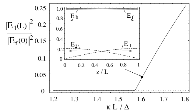
FIG. 2. Phase transition to mirrorless parametric oscillations. Analytic solution for amplitude of generated field for \gamma_0 = 0 . Insert: Normalized field amplitudes inside medium for E/|E_f(0)| = 0.2
