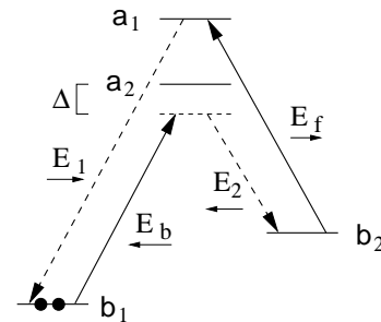
FIG. 1. Atoms in double \Lambda configuration interacting with two classical driving fields in forward ( E_f ) and backward direction ( E_b ) and two quantum fields ( E_{1,2} ). All optical transitions are assumed to be radiatively broadened.
