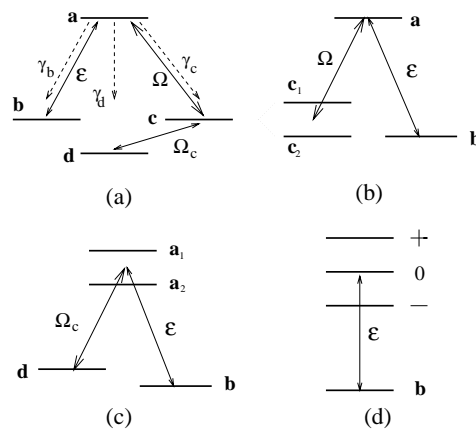
FIG. 1. (a) Four state system displaying double-dark resonances. Unitary equivalent systems: (b) corresponds to generic model Fig. 1a after diagonalizing the interaction with the coherent perturbation \Omega_c (states |c_1\rangle and |c_2\rangle correspond to (|c\rangle \pm |d\rangle)/\sqrt{2} , respectively) and (c) after diagonalizing the interaction with the drive field \Omega (states |a_1\rangle and |a_2\rangle correspond to a pair (|a\rangle \pm |c\rangle)/\sqrt{2} displaying Fano interference due to spontaneous emission) (d) Dressed state picture corresponding to the Figs. a,b,c.
