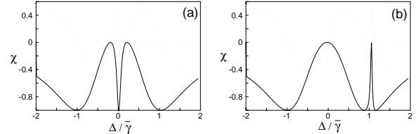
FIG. 2. Imaginary (solid lines) and real (dashed lines) parts of the probe susceptibility in the units of \eta/\bar{\gamma} for a system of Fig. 1a. Parameters are \gamma_b = \gamma_c = \gamma_d = \bar{\gamma} , \Omega = \bar{\gamma} , \Omega_c = 0.2\bar{\gamma} , r = \gamma_0 = 0 , \Delta_0 = 0 . (a) \Delta_c = 0 . (b) \Delta_c = \bar{\gamma} . Case (b) is the special case when the dressed energies intersect ( E(|-\rangle) \sim E(|0\rangle) ).
