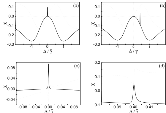
FIG. 3. Imaginary (solid lines) and real (dashed lines) part of the susceptibility in the units of \eta/\bar{\gamma} for (a,c) optical gain and (b,d) enhanced index of refraction without absorption. The parameters are \gamma_b = \gamma_c = \gamma_d = \bar{\gamma} , \Omega = \bar{\gamma} , \Omega_c = 0.01\bar{\gamma} , \gamma_0 = 3r_b = 3r_c = 3r_d = 0.0001\bar{\gamma} , and r = 0.001\bar{\gamma} , \Delta_c = 0 for (a,c) and r = 0.0005\bar{\gamma} , \Delta_c = 0.4\bar{\gamma} for (b,d).
