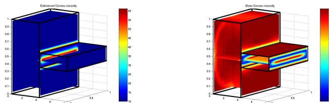
Figure 3: 3D planar contraction geometry. Extensional viscosity (left figure) and shear viscosity (right figure).
