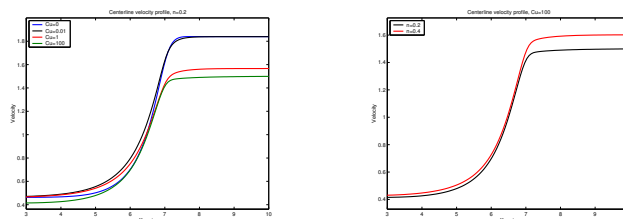
Figure 1: The effect of varying Cu number on the calculated centerline velocity for n=0.2 , Carreau model (left plot). The effect of varying n number on the calculated centerline velocity for Cu=100 , Carreau model (right plot).
