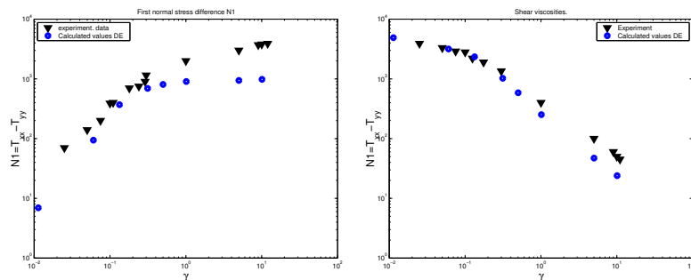
Figure 7: Rheological results for polystyrene solution. Left figure presents comparison of N_1 = T_{xx} - T_{yy} between the experimental data (black triangles) given in [6] and calculated results (blue circle) against shear-rate \dot{\gamma} . Right figure presents comparison of the shear viscosity, defined as \eta(\dot{\gamma}_{xy}) = \frac{T_{xy}}{\dot{\gamma}_{xy}} , against shear-rate \dot{\gamma}_{xy} between experimental measurements and calculated results.
