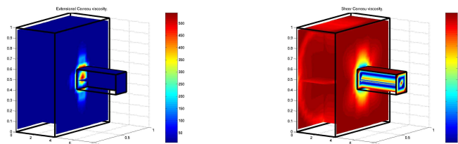
Figure 5: 3D square-to-square contraction geometry. Extensional viscosity (left figure) and shear viscosity (right figure).
