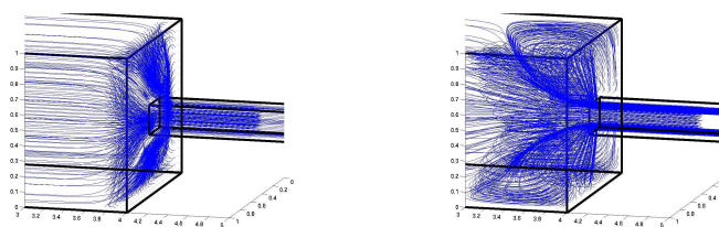
Figure 4: 3D square-to-square contraction geometry. Streamline plots, Newtonian fluid (left figure) and extensional-thickening fluid (right figure).
