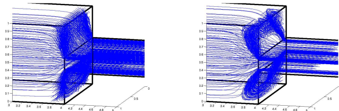
Figure 2: 3D planar contraction geometry. Streamline plots, Newtonian fluid (left figure) and extensional-thickening fluid (right figure).
