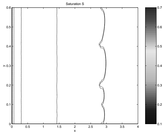
Figure 2. Distribution of gas saturation. Viscous fingers are triggered by the modified permeability field.
