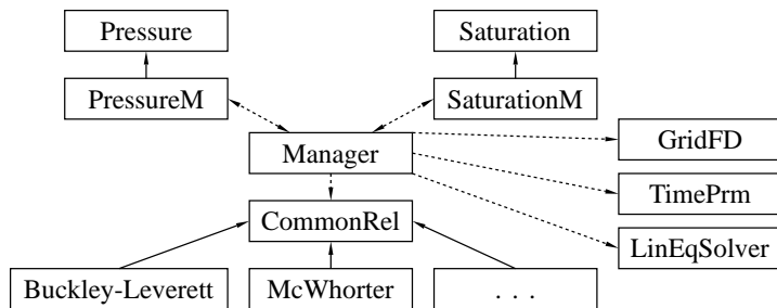
Figure 1. Design of the PDE system solver with relations between solver classes, manager and pool of common relations. Solid arrows indicate inheritance ("is-a" relationship, with arrows pointing from subclass to base class). Dashed arrows indicate pointer ("has-a" relationship).
