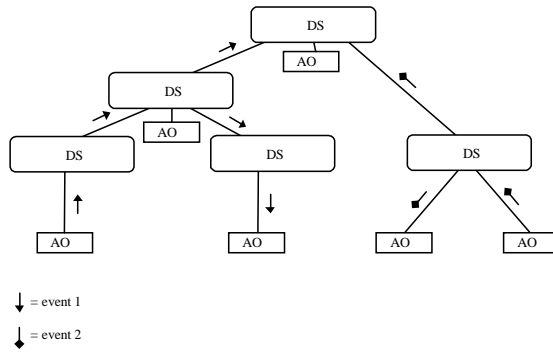
Figure 3: The JEDI architecture with the distributed ED
