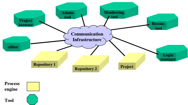
Figure 1: The PROSYT logical architecture.
