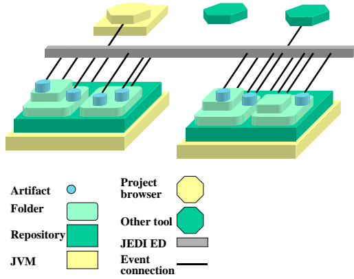
Figure 4: The physical architecture of the first PROSYT prototype.
