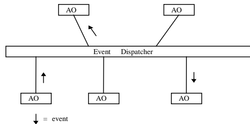
Figure 2: A logical view of JEDI architecture.
