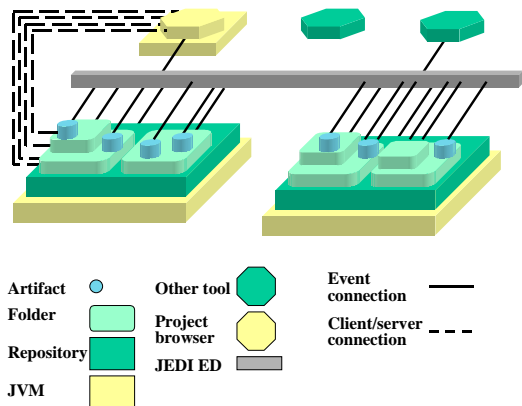
Figure 6: The physical architecture of the second PROSYT prototype.
