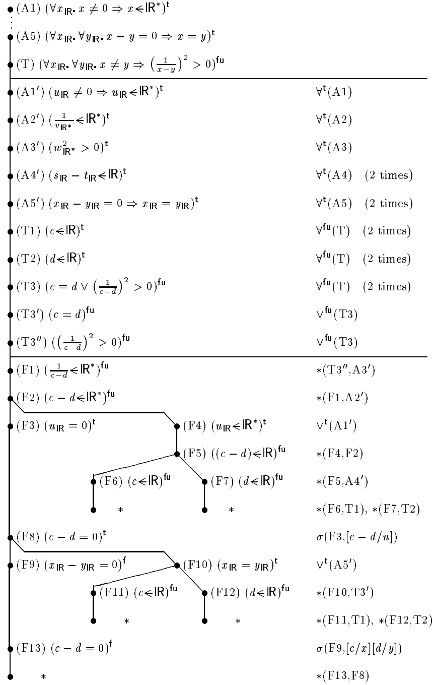
Fig. 1. Tableau proof with unsorted unification, example 3.7
