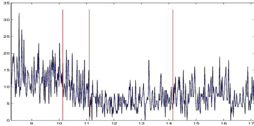
Figure 6.11: Stock Ericsson B: July 3rd 2002 and possible change points (by binary segmentation)
