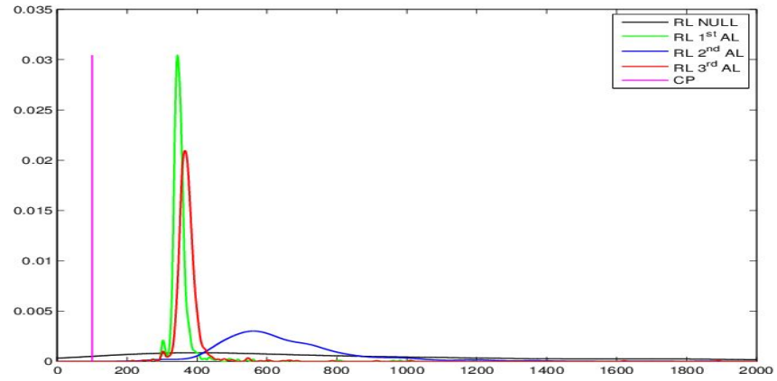
Figure 6.4: RL density estimate, m=200
