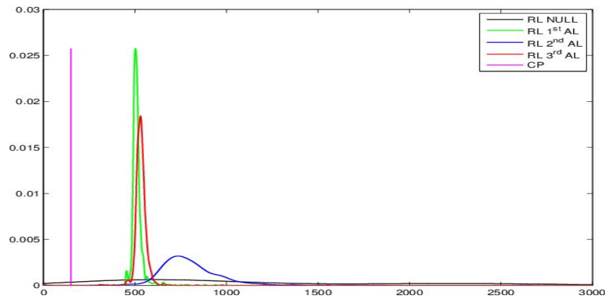
Figure 6.5: RL density estimate, m=300
