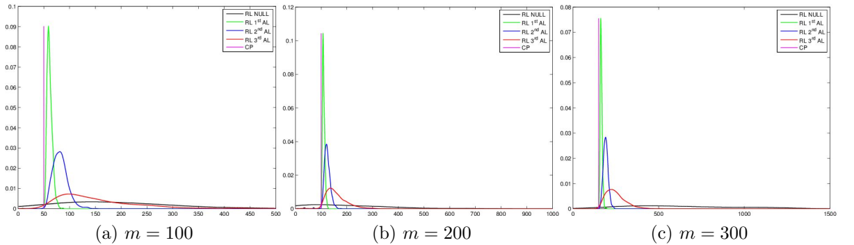
Figure 6.10: Scaled density estimate of the run length for BAR(1)-model
