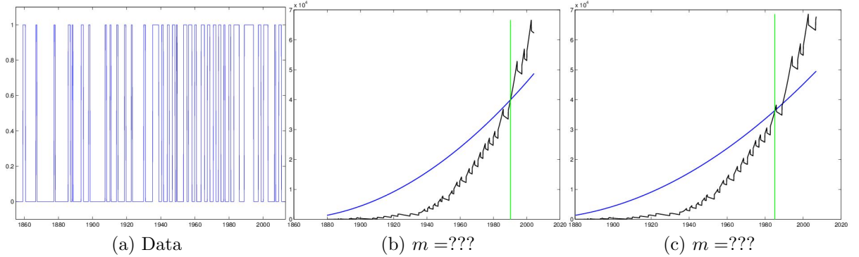
Figure 6.9: Monthly US Recession data (1855-2013) and its detectors
