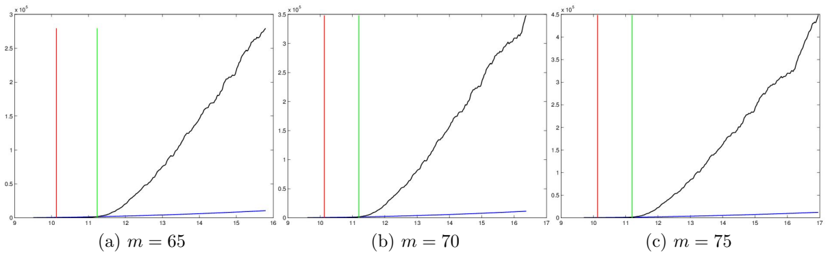
Figure 6.12: Value of the detector of change for the number of transaction per minute of the Ericsson B stock data with different start dates for the monitoring
