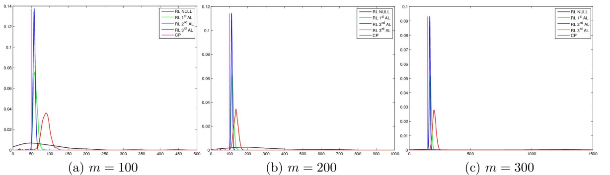
Figure 6.8: Scaled density estimate of the run length for BAR(1)-model
