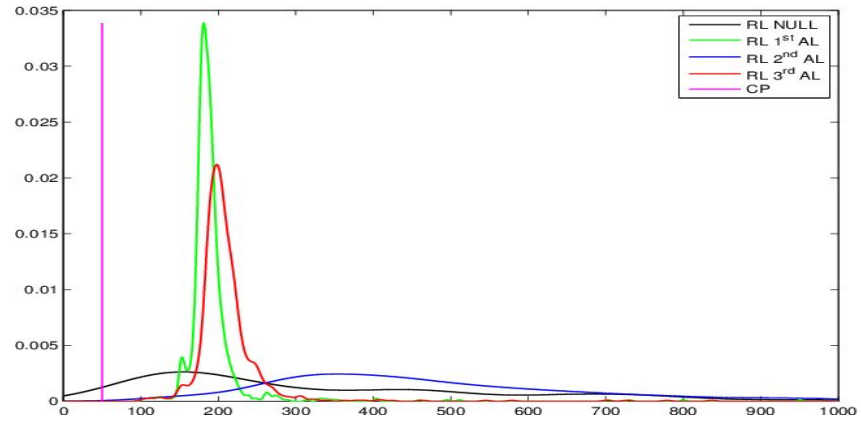
Figure 6.3: RL density estimate, m=100
