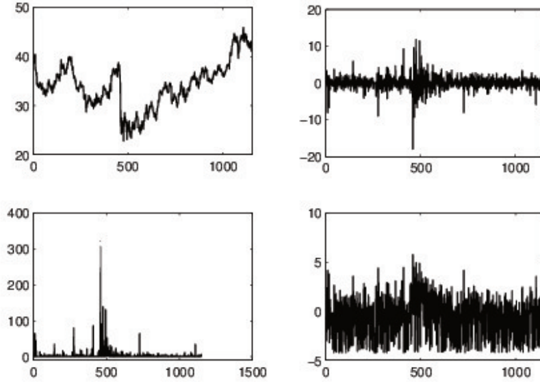
Figure 6.6: SAP stock returns and suitable transformations (January 2007 to April 2011)
