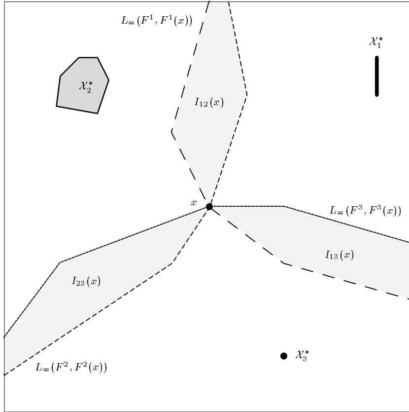
Figure 7: Illustration to the proof of Lemma 4.1
