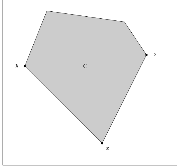
Figure 4: Illustration to Lemma 3.1: y, x, z \in \text{Ext}(C) in counterclockwise order
