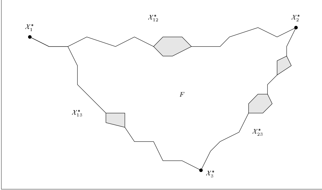
Figure 6: Illustration to Lemma 4.1
