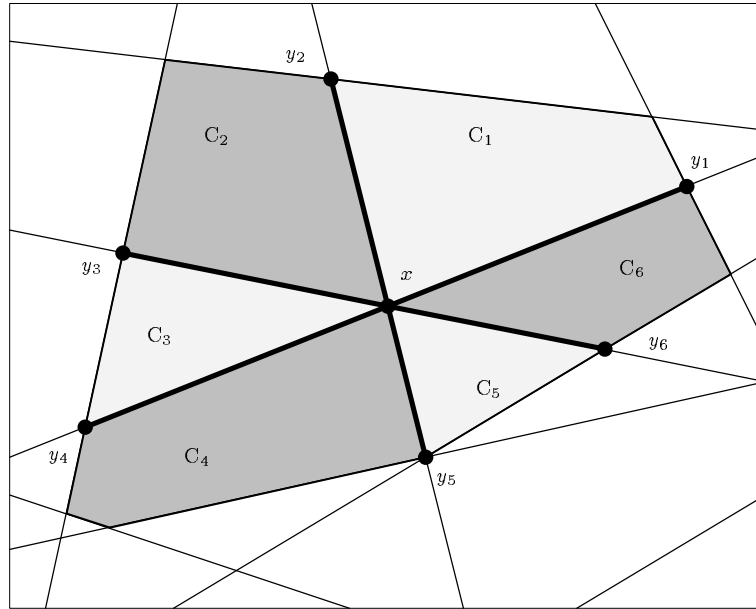
Figure 5: Illustration to Lemma 3.2 with P_x = 6
