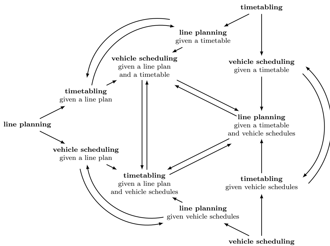
Figure 3.1: Depiction of the eigenmodel described in [24].
