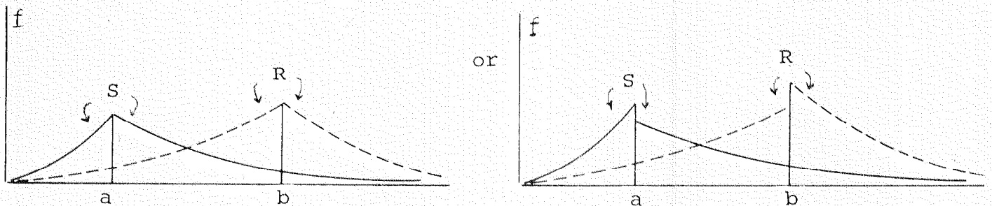
Fig. 2. Combined Power-Pareto distributions for R and S
