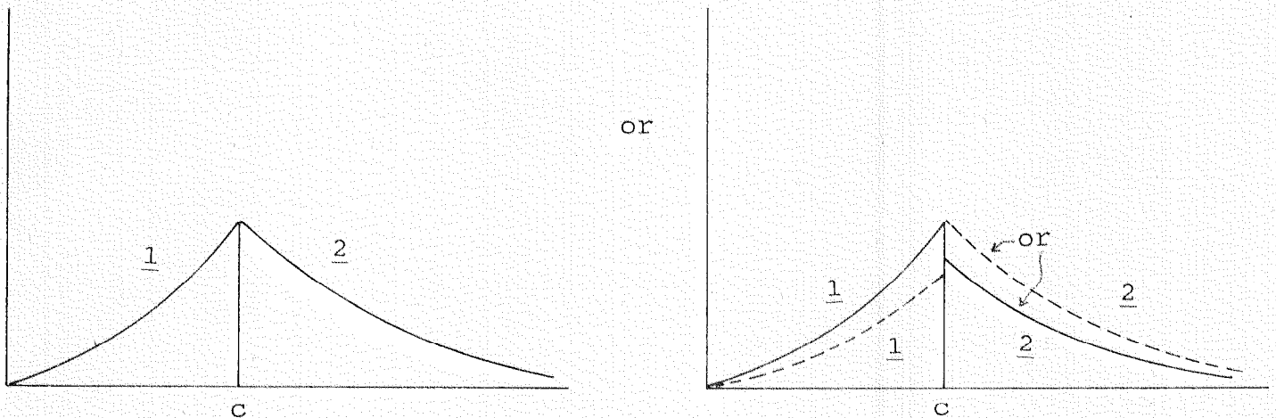
Fig. 1. Illustration of Power and Pareto distributions
