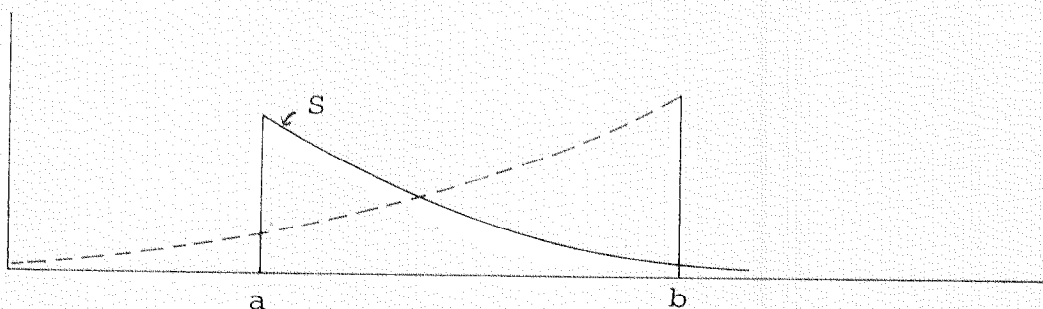
Fig. 3. Power/Pareto tail models for R and S
