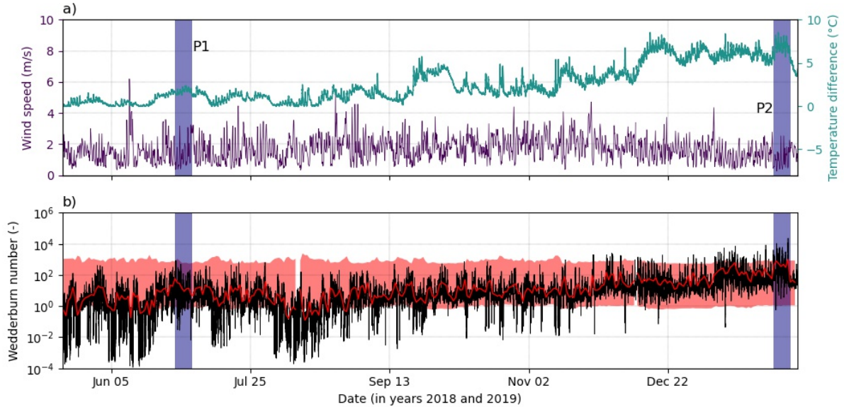
Figure 20 – Conditions at Passaúna reservoir during the monitoring period. a) 3-h average wind speed measured at the meteorological station near the dam (purple solid line) and temperature difference between the water surface and the bottom (green solid line). b) Wedderburn number ( W ) calculated with 3-h resolution (black solid line) and averaged over one internal seiche period (red solid line). The red background color marks the range of W , for which internal seiche dominance is predicted by a common classification scheme (Fig. 49). The vertical blue bars indicate the two analysis periods (P1, from June 28 to July 04), and P2 (from January 29 to February 04).
