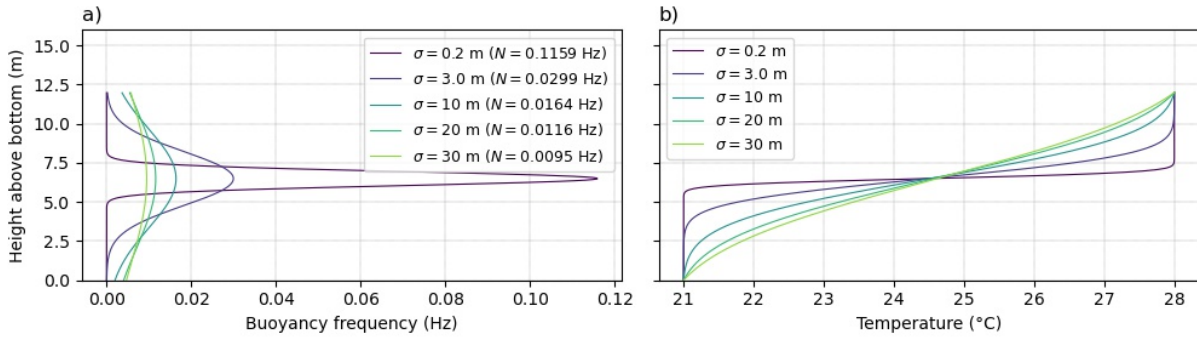
Figure 19 – Vertical profiles of density stratification used in the numerical simulations. a) Buoyancy-frequency ( N ) and b) temperature profiles for different values of \sigma (the standard deviation describing the Gaussian form of the buoyancy-frequency profile). N refers to the maximum buoyancy frequency of each stratification profile.
