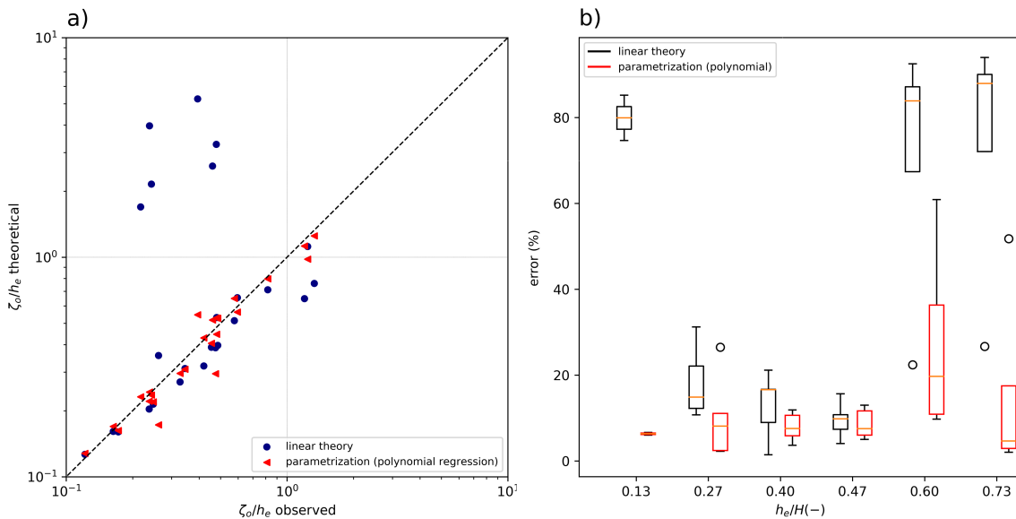
Figure 15 – a) Comparison between theoretical (linear and parametrized equation) and internal seiche amplitude detected in simulations. b) Error percentage with respect to h_e/H .
