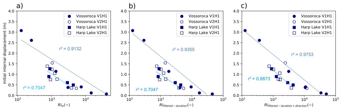
Figure 10 – Internal seiche amplitude of the most energetic isotherm versus a) the daily Ri_w , b) filtered Ri_{duration} using only periods with winds capable to generate internal waves, and c) filtered Ri_{direction} using only periods with winds in directions capable to generate internal waves. Linear regression was obtained for each basin
