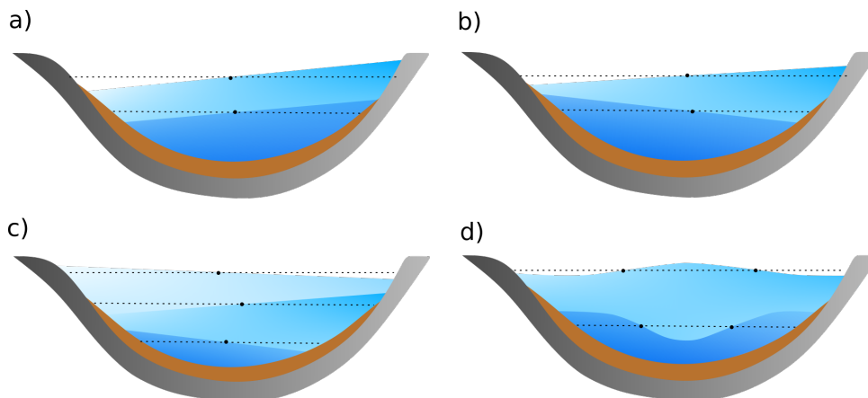
Figure 4 – Schematic view of various internal wave modes in a closed basin: a) V_0H_1 , b) V_1H_1 , c) V_2H_1 and d) V_1H_2 . The mode for n = 0 is related to the pure surface (barotropic) mode. The black dots (·) represent nodal points
