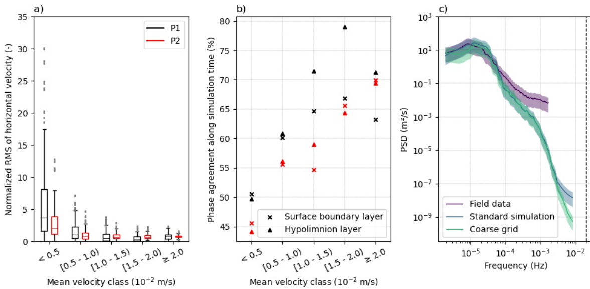
Figure 48 – Comparison of measured and simulated horizontal flow velocities for period P1 (weaker stratification) and P2 (stronger stratification). a) Normalized root mean square difference (NRMSD) of the horizontal velocity difference between measured and simulated data for different velocity classes for period P1 (black) and P2 (red). The boxes extend over the 25th and 75th quartiles, whilst the horizontal line indicates the median value. The whiskers extend to the minimum and maximum values neglecting outliers, which are represented by gray dots. b) Period of time (in percentage) that the direction of simulated horizontal velocities agreed with measured data for both periods and for different velocity classes. Crosses and triangles represent data from near the reservoir bottom (2.5 m above the bottom) and near the water surface (9 m above the bottom), respectively. c) Power spectral density of horizontal velocity variations at approximately 2.5 m above the bottom for measured (purple) and two simulations (blue and green). The solid blue line represents the spectral density of simulations using the standard grid size of our scenario analyses, whilst the solid green line represents PSD obtained from a coarser numerical grid. The colored shaded area shows the 95% confidence interval.
