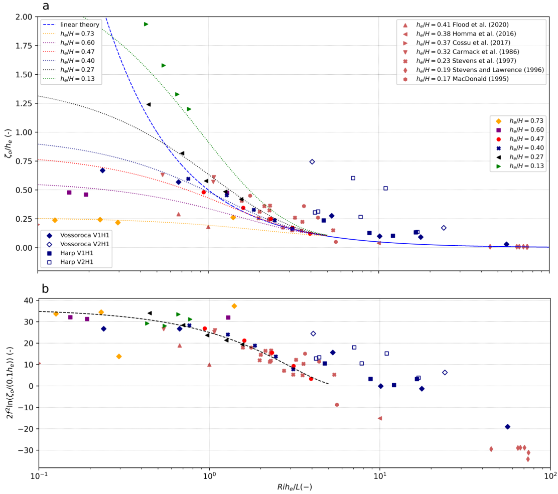
Figure 16 – a) Maximum vertical displacement associated with internal seiche normalized by the epilimnion thickness against Ri h_e/L . Data points include values from simulations, Harp lake, Vossorooca reservoir, and many other lakes from the literature (FLOOD et al., 2020; HOMMA et al., 2016; COSSU et al., 2017; CARMACK et al., 1986; STEVENS; LAWRENCE, 1997; STEVENS et al., 1996; MACDONALD, 1995) b) Normalization of \zeta_o/h_e to incorporate the function f(h_e/H) ( 2f^2 ) against Ri h_e/L . The black dashed line represents Eq. 2.8 normalized by 2f^2 . "Log" is defined in base e, natural logarithm.
