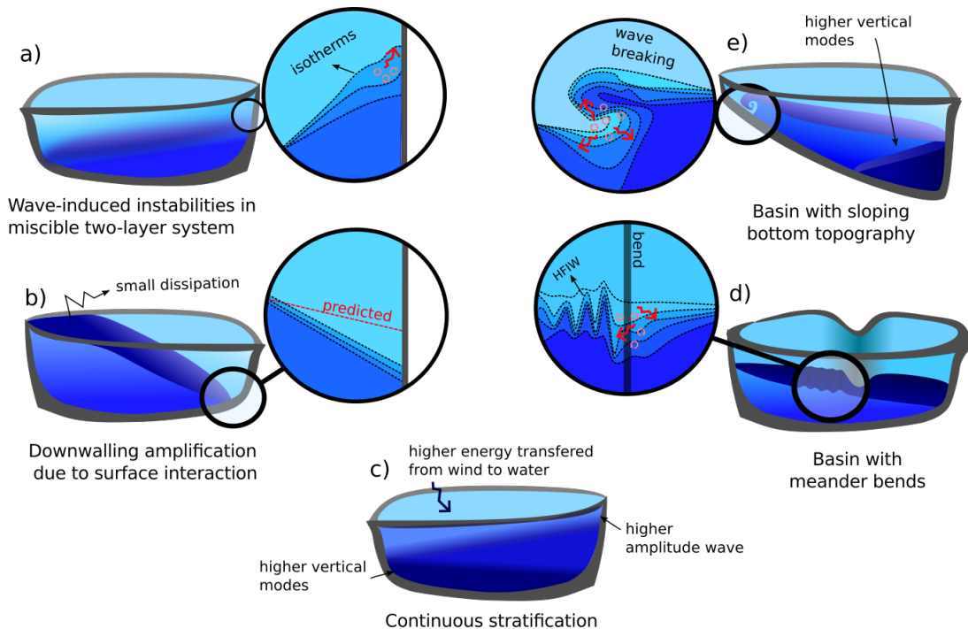
Figure 38 – Summary of the main findings related to the mechanism of wave dissipation observed during upwelling events and internal seiche activity. Explanations are provided in the text.
