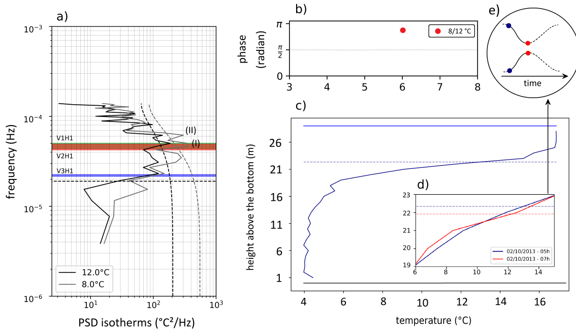
Figure 41 – a) Power spectral density of the isotherms of 12 °C and 8 °C. Dashed lines show the mean red noise spectrum for the time series, indicating significant peaks at a 95% confidence level. b) spectral phase analyses considering just coherence higher than 80% (Harp Lake; 25/09 – 05/10), c) Vertical temperature profile obtained from Harp Lake in 2nd of October 2013 at 5 a.m., d) Zoom-in view of the temperature profile with a second profile 2 h late, which is approximately half of the internal seiche period. At 22 m above the bottom the water becomes warmer, which leads to an erosion of the 12 °C isotherm due to internal seiche passage. However, 2 m below that point, the water becomes colder due to the elevation of the 8 °C isotherm, that was caused by the oscillation of the second interface, clearly out-of-phase with the 12 °C isotherm. e) a sketch of the V2 mode that is presented in item (d).
