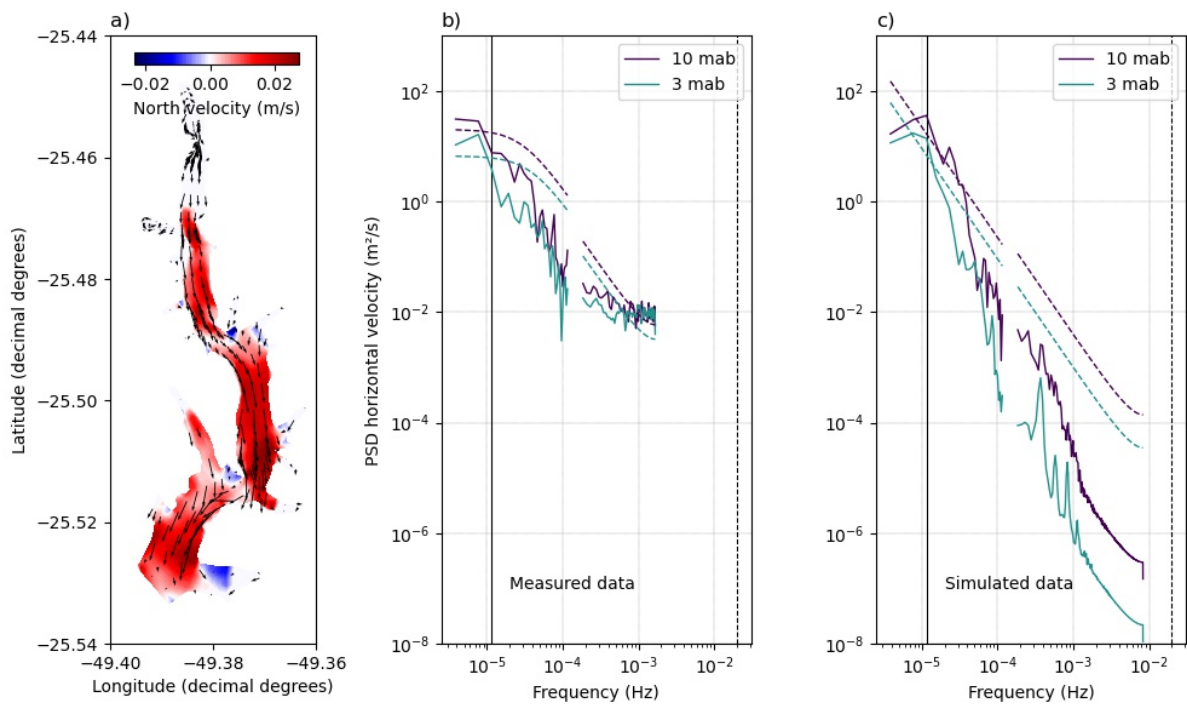
Figure 43 – Hydrodynamic characterization of the analyzed period P1. a) Simulated horizontal flow velocity during the upwelling event on June 29 (2018) at 17 : 00 h. The black arrows illustrate the horizontal velocity direction and magnitude near the water surface (2 m depth). The color scaling shows opposing (northward) flow in the hypolimnion (8 m above the deepest part of the reservoir). Power spectral density of b) observed, and c) simulated time series of horizontal flow velocity at two different depths at the monitoring station (red dot in Fig. 18a in the main text). For low-frequencies ( 10^{-6} to 10^{-4} Hz), the spectra were calculated with a window size of 3 d, while in the high-frequency range (up to 10^{-4} Hz), we used a window size of 12 h. The dashed lines show the 95% confidence limit of the mean red noise spectrum estimated for each time series. The vertical black dashed line marks the buoyancy frequency ( N = 0.02 Hz), and the vertical solid black line shows a 24-h period.
