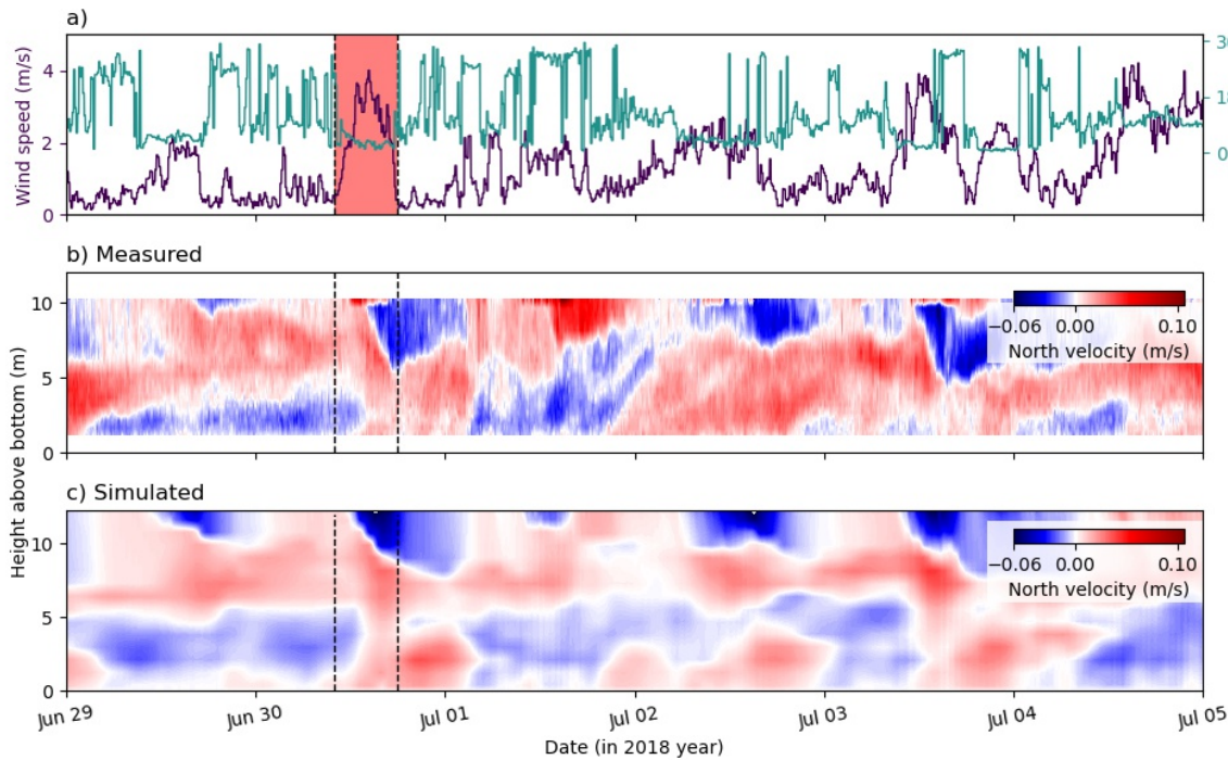
Figure 21 – a) Wind speed (purple line) and wind direction (green line) during the analysis period P1. The red shaded area, delimited by vertical black dashed lines, marks a solitary wind event that may favor the generation of internal seiches. b) Measured, and c) simulated horizontal flow velocities in south to north direction at the location of the monitoring station (Fig. 18a) with a temporal resolution of 1 min.
