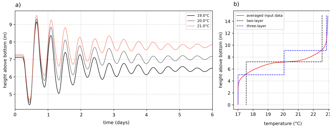
Figure 30 – a) Time series of selected isothermal depths at the sampling point ST in the numerical simulations. b) Temporarily averaged vertical temperature profiles /red line) and the two (black line) and three-layer (blue line) approximation of the temperature profiles used for modal internal wave analysis.
