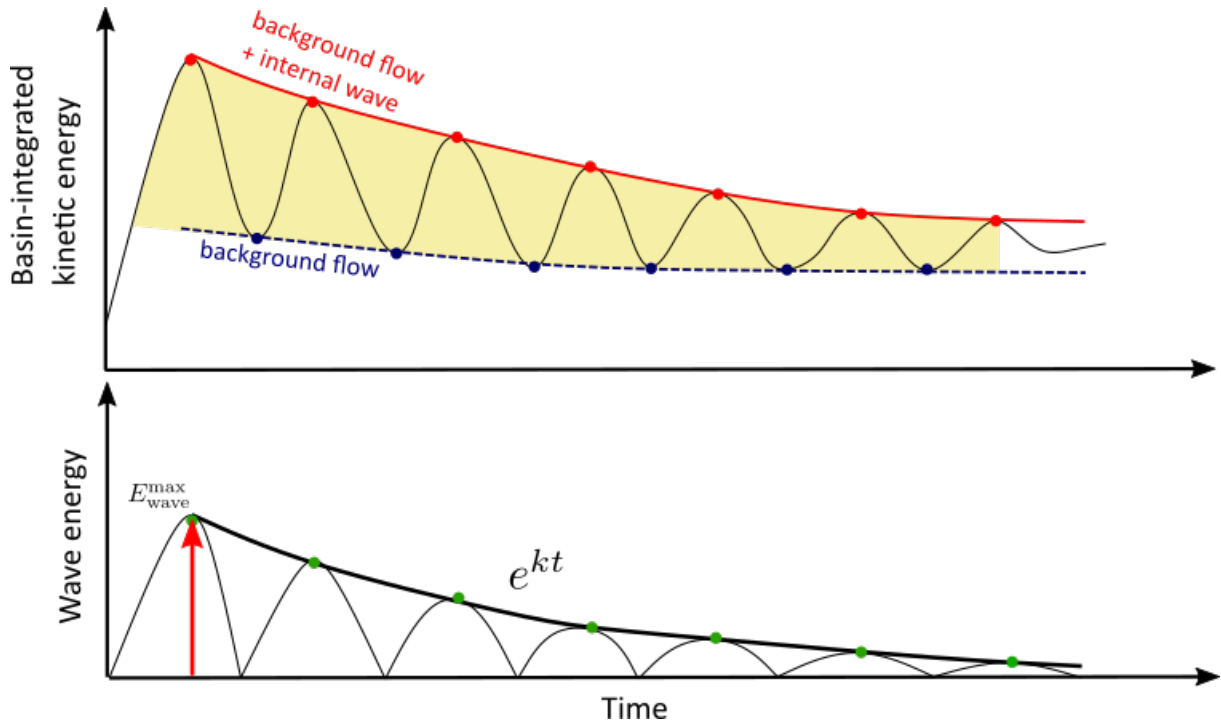
Figure 50 – Time-series of internal wave energy ( E_{wave} ) and the procedure to remove the background flow from the basin-integrated kinetic energy (Eq. 3.2 in the main text). Red and blue dots represent the identified maximum and minimum values from the time-series of basin-integrated kinetic energy, respectively. Red solid and blue dashed lines represent the total energy decay and the background flow decay, respectively. Green blue dot is the internal wave energy obtained from the difference between the basin-integrated kinetic energy (red dots) and the function of the background flow energy (blue dashed line), in which the first green dot (red arrow) describes the initial energy of the internal wave ( E_{wave}^{max} ). k is the internal wave damping coefficient (Eq. 3.3 in the main text).
