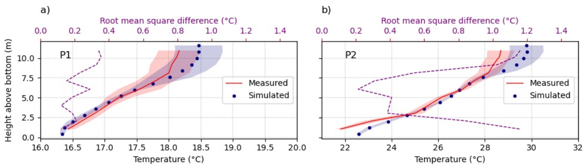
Figure 47 – Vertical stratification during the analysis periods at the sampling site near the intake station (Fig. 18a in the main text): a) P1 (from June 28 to July 04, 2018) and b) P2 (from January 29 to February 04, 2019). Both panels show the mean vertical profiles of simulated (blue dots) and measured (red solid line) temperature, with their standard deviations marked by the blue and red shaded areas. The purple dashed lines show the root mean square difference between simulations and observations.
