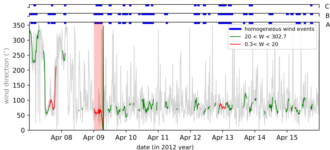
Figure 35 – Time series of wind direction at Vossoroça reservoir (grey line). The blue bars above the graph indicates periods of constant wind directions according to three different angles of wind direction contribution: A: \pm 20^\circ , B: \pm 40^\circ , and C: \pm 5^\circ . Periods marked by green and red color correspond to criteria suggesting internal wave generation. The green line represents the more flexible criteria often described by mathematical results from Spigel and Imberger (1980). The red line indicates a more restrictive result, which fall into regime of internal wave described by Spigel and Imberger (1980) and often observed from field data reported in the wide literature. The value of W_{V1} displayed in the label indicates an average for the entire period, and just illustrates the mean value of the adopted criteria. The vertical red bar indicates the period in which the internal wave was generated.
