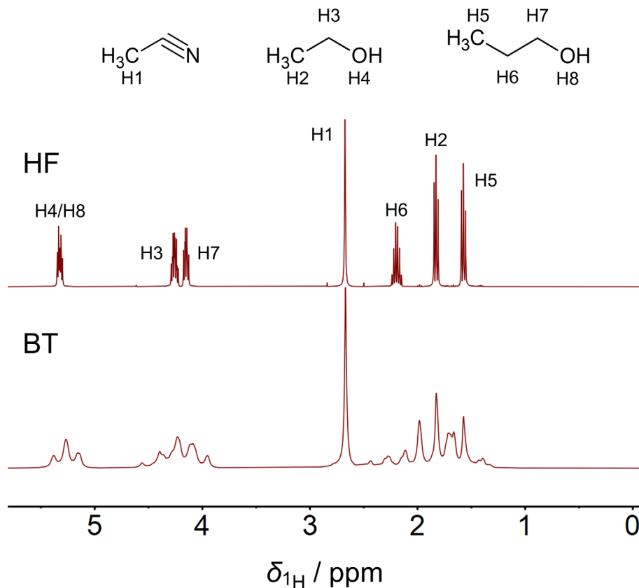
FIGURE 3 Comparison of 1 H NMR spectra of an equimolar mixture of MeCN + EtOH + PrOH acquired in a high-field (HF, top) and a benchtop NMR spectrometer (BT, bottom). Also the peak assignment is indicated.
