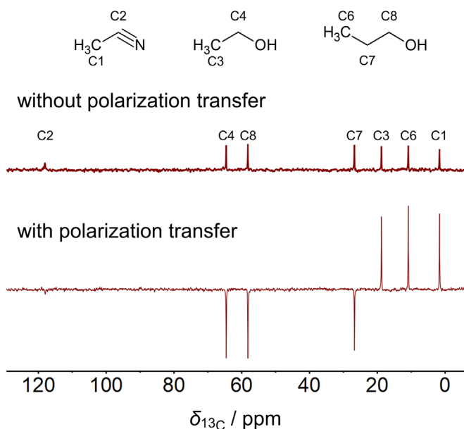
FIGURE 4 Comparison of 13 C NMR spectra of an equimolar mixture of MeCN + EtOH + PrOH acquired without (top) and with the polarization transfer sequence PENDANT (bottom) in a benchtop NMR spectrometer. Also the peak assignment is indicated.
