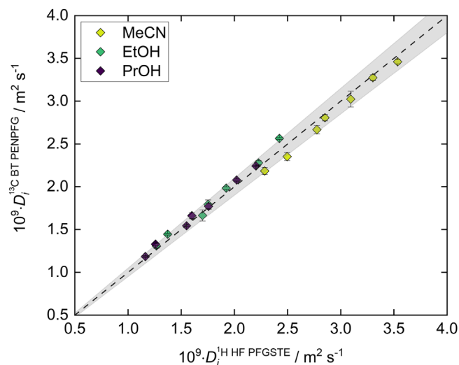
FIGURE 7 Self-diffusion coefficients of MeCN, EtOH and PrOH in ternary mixtures of MeCN + EtOH + PrOH at T = 301.65 K measured with ^{13}\text{C} BT PENPFG. The parity plot compares the results from ^{13}\text{C} BT PENPFG to the reference values from ^1\text{H} HF PFGSTE. The grey shaded area indicates relative deviations below 5%.
