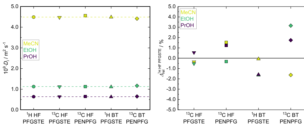
FIGURE 5 Left: Comparison of the experimental results of different NMR techniques for the self-diffusion coefficients of the pure components MeCN, EtOH and PrOH at T = 301.65 K. The symbols indicate results obtained with the different methods and instruments (HF high-field, BT benchtop; PFGSTE standard experiment, PENPFG experiment with polarization transfer). The dashed horizontal lines represent the reference measurement with ^1\text{H} HF PFGSTE. All error bars are within the symbol size (further details are given in the Supporting Information). Right: Relative deviations of the results obtained by different NMR techniques compared with the reference method ^1\text{H} HF PFGSTE.
