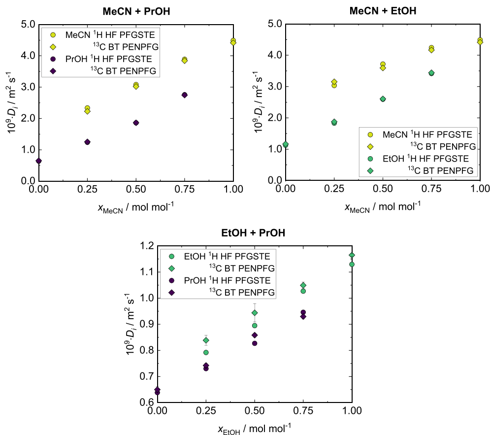
FIGURE 6 Comparison of results of measurements of self-diffusion coefficients of MeCN, EtOH and PrOH in the binary mixtures MeCN + PrOH, MeCN + EtOH and EtOH + PrOH at T = 301.65 K. The diamonds stand for results obtained with ^{13}\text{C} BT PENPFG, the circles for the results from ^1\text{H} HF PFGSTE. For the binary mixture EtOH + PrOH, the vertical scale is magnified by a factor of 10. Error bars are only shown if they are larger than the symbol size.
