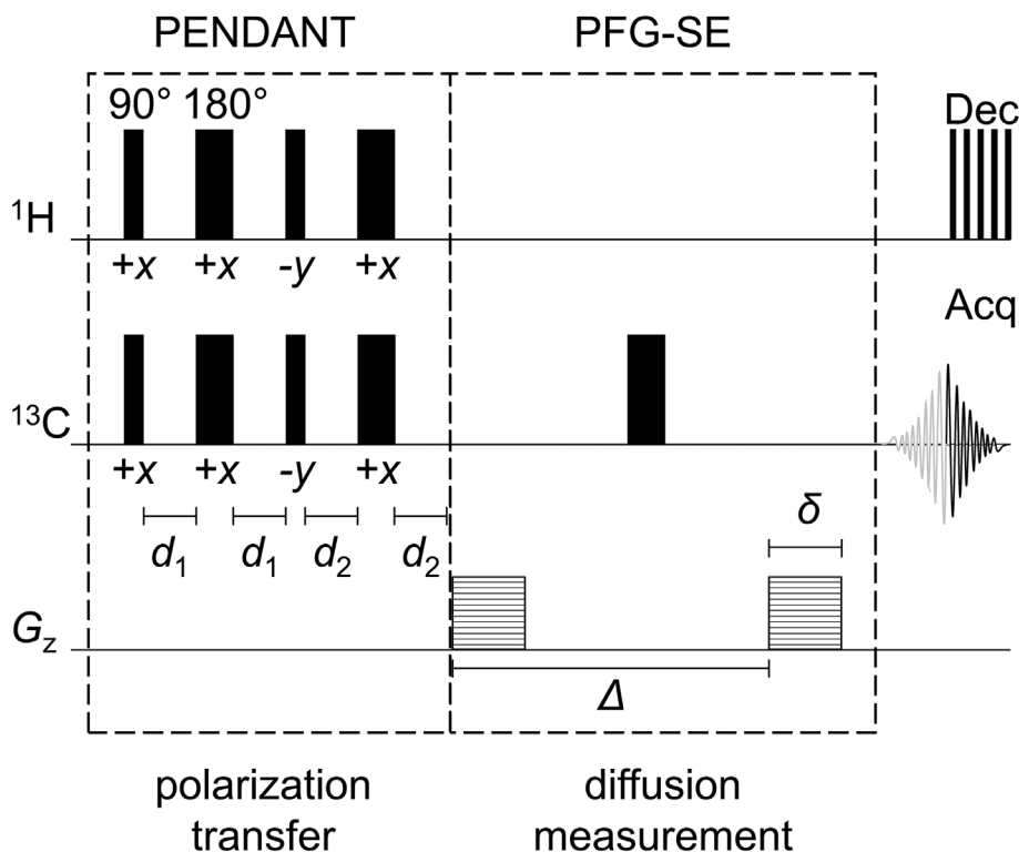
FIGURE 1 Illustration of the PENPFG pulse sequence for the measurement of self-diffusion coefficients with ^{13}\text{C} NMR spectroscopy, consisting of the polarization transfer pulse sequence PENDANT for signal enhancement and the PFG-SE sequence for diffusion encoding. The delays d_1 and d_2 depend on the ^{13}\text{C} - ^1\text{H} ^1J_{\text{C,H}} -coupling constants. \Delta denotes the diffusion time and \delta the gradient pulse duration.
