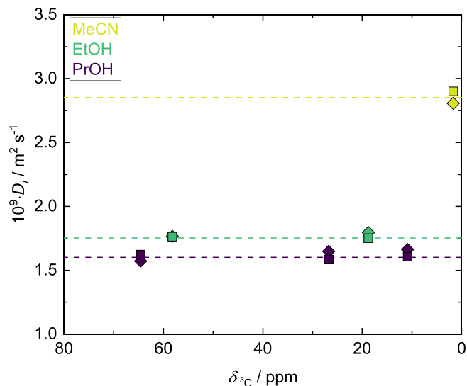
FIGURE 8 DOSY representation of an equimolar mixture of MeCN + EtOH + PrOH at T = 301.65 K. The squares and diamonds indicate results from ^{13}\text{C} HF PENPFG and ^{13}\text{C} BT PENPFG. The dashed horizontal lines represent the reference measurement with ^1\text{H} HF PFGSTE, obtained by the analysis of the \text{CH}_3 group of the specific molecules. All error bars are within the symbol size.
