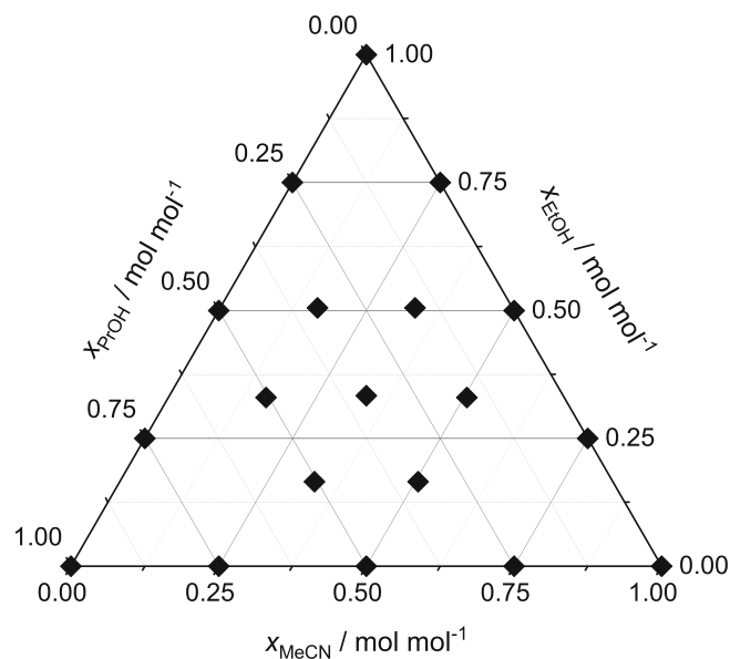
FIGURE 2 Overview of the studied mixtures consisting of acetonitrile (MeCN), ethanol (EtOH) and 1-propanol (PrOH).
