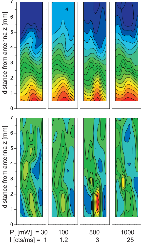
Fig. 1: Distribution of the spin wave intensity |\varphi|^2 normalized to the maximum intensity at minimum measured distance to the antenna of 0.5mm . The microwave input power and the absolute values of the light scattering intensity, measured near the input antenna, are indicated in the figure. The mode propagation is from bottom to top on each panel. The upper panels show the raw data in a logarithmic scale. In the lower panels |\varphi|^2 \cdot \exp(\kappa z) is shown in a linear color scale.
