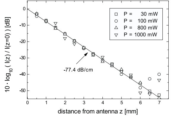
Fig. 2: Integrated intensity of the spin wave modes I(z) as a function of the distance to the antenna normalized to its extrapolated value at z = 0 . The attenuation parameter obtained from a fit (full line) is \kappa = 77.4 \pm 1.5 dB/cm .
