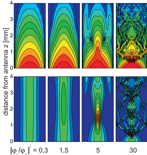
Fig. 3: Numerically calculated stationary distribution of the spin wave intensity. Upper panels show |\varphi(y, z)|^2 normalized to the maximum intensity |\varphi_0|^2 of the initial ( z = 0 ) beam intensity distribution in a logarithmic scale. Lower panels show |\varphi/\varphi_0|^2 \cdot \exp(\kappa z) in a linear scale.
