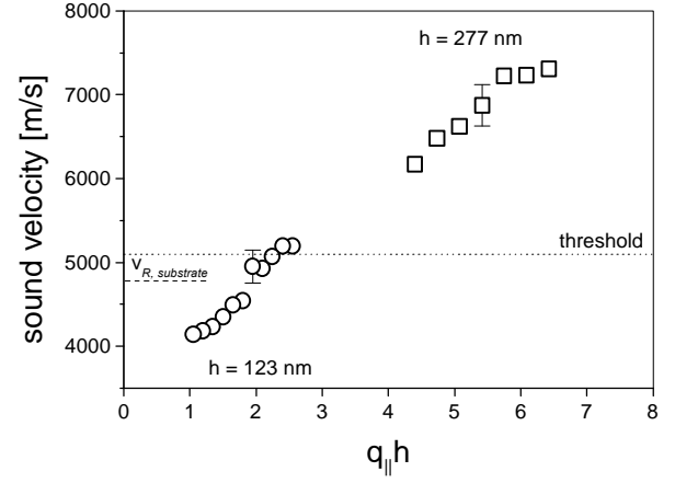
Fig. 3: Measured sound velocities of the surface modes of two c-BN films as in Fig. 1 versus the product of wavevector q_{\parallel} and film thickness h . The sound velocities of the thicker film (squares) lie far above the velocity threshold indicated by the dotted line. The sound velocities of the thinner film (circles) lie below the threshold and reach the threshold at q_{\parallel}h \approx 2.5 . The dashed line on the left indicates the Rayleigh velocity v_{R,\text{substrate}} of the (111) silicon substrate in [110]-direction.
