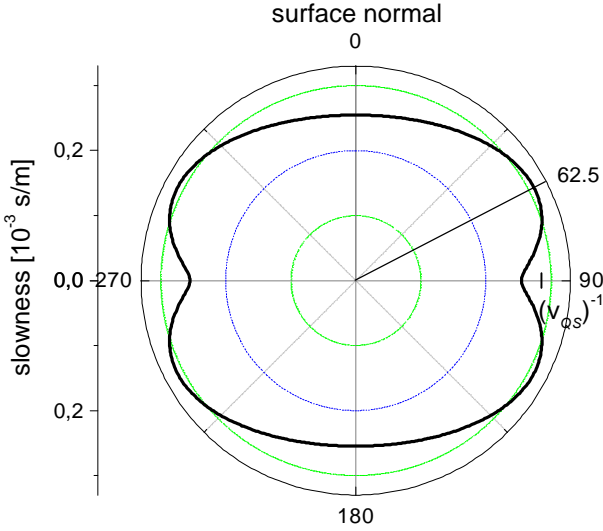
Fig. 2: Polar plot of the intersection of the slowness surface of the quasi-shear wave with any meridian plane for the r.f. sputtered sample. Pure modes propagate with the angles 0^\circ , 62.5^\circ and 90^\circ inclined to the surface normal. The projection of the curve on the direction of propagation parallel to the surface yields (v_{QS})^{-1} . For large wavevectors the velocities of all Sezawa modes converge against the velocity limit v_{QS} (see Fig. 1).
