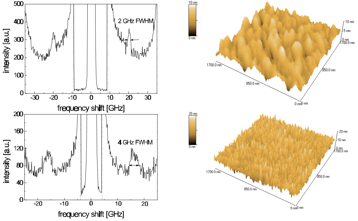
Fig. 4: Brillouin light scattering spectrum and surface topography of the 150 nm thick BN film (top) and the 75 nm thick h-BN film (bottom). The dotted lines in the spectra indicate the frequency range of the suppressed elastically scattered light. The energetic width of the Rayleigh mode, which is visible both on the Stokes and Anti-Stokes side of the spectra, correlates with the grain sizes at the surface of the samples.
