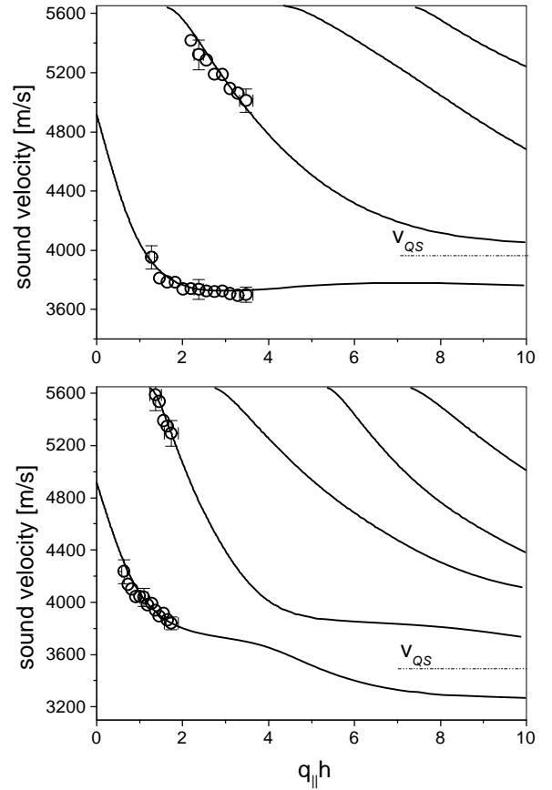
Fig. 1: Measured (open circles) and fitted (lines) sound velocities of the BN film modes versus the product of wavevector q_{\parallel} and film thickness h . The upper and lower diagram show the dispersion of the r.f. sputtered film ( h = 75 \text{ nm} ) and of the d.c. sputtered film ( h = 150 \text{ nm} ), respectively. Vertical error bars are due to the finite accuracy of the frequency determination in the BLS spectra, horizontal error bars are due to the finite accuracy in the determination of the film thickness. The phonon wavevector is varied by the angle of light incidence. The curves show the results of a least squares fit to the experimental data with the elastic constants as free parameters. The dotted line indicates the velocity of the quasi-shear bulk mode v_{QS} , travelling parallel to the surface.
