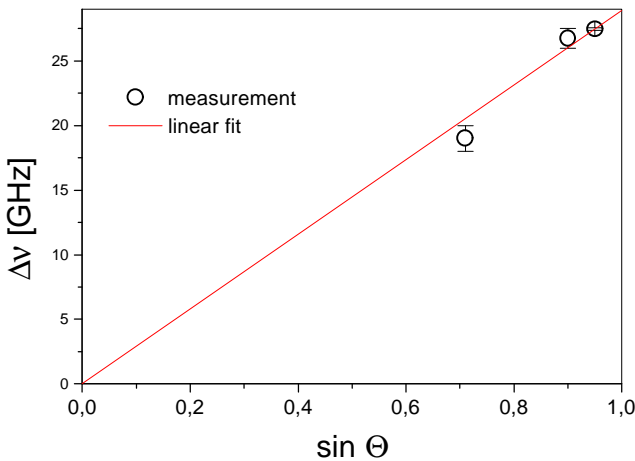
Fig. 5: Phonon frequency versus \sin \theta for a 600 nm thick c-BN film. The sound velocity of the surface wave is not influenced by the material at the interface or the substrate due to the large film thickness. From the slope of the linear fit the Rayleigh mode sound velocity is v_R = 7440 \pm 419 m/s.
