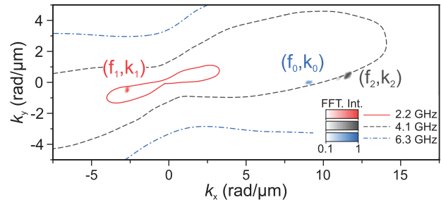
Figure 4. Scheme of first-order instability process. The color patches show the simulated spin-wave intensity while the lines show the isofrequency curves for frequencies f_0 to f_2 . The magneto-elastic field is driven with f_0 = 6.3 \text{ GHz} (blue) and leads to pumping of the spin-wave modes f_1 = 2.2 \text{ GHz} (red) and f_2 = 4.1 \text{ GHz} (black) while conserving momentum and energy.
