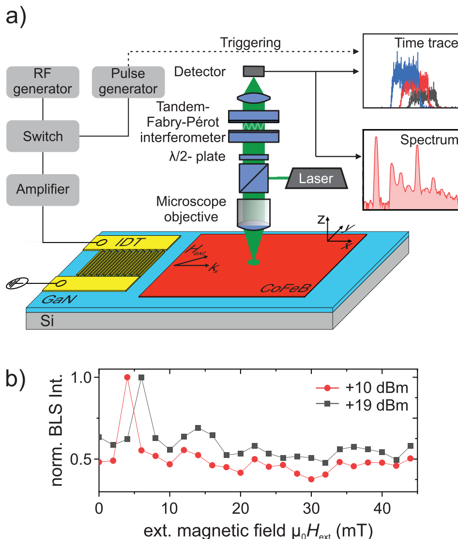
Figure 1. a) Schematic illustration of the experimental setup. SAWs are excited by the IDT and propagate toward a 350 \times 350 \mu\text{m}^2 square pad made from a \text{Co}_{40}\text{Fe}_{40}\text{B}_{20} thin film with thickness h_{\text{CoFeB}} = 18 \text{ nm} . b) Normalized BLS intensity at the frequency of the fundamental mode f_0 = 6.3 \text{ GHz} as a function of the applied magnetic field for the linear and non-linear case. The maxima correspond to the resonant excitation of spin waves by the SAWs. The change in the resonance field with power is caused by the nonlinear shift.
