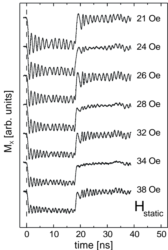
Figure 2: Time evolution of the x-component of the magnetization, M_x , measured at the center of the sample during and after field pulse excitation for different static magnetic field values, H_{\text{static}} , as indicated. The magnetic field pulse is 1.6 Oe and the pulse duration is 18 ns. The beginning of the pulse launch is at time t = 0 ns.
