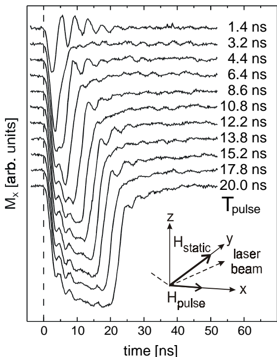
Figure 1: Time evolution of the x-component of the magnetization, M_x , measured at the center of the sample during and after field pulse excitation for different pulse durations, T_{\text{pulse}} , as indicated. The static magnetic field is 4 Oe, the magnetic field pulse 0.6 Oe. The beginning of the pulse launch is at time t = 0 ns. Inset: Coordinate system and geometry of the experiment.
